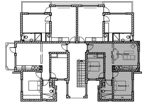
Ground Floor Key Plan Unit No. 104
