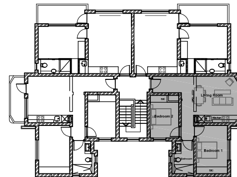
Third Floor Key Plan Unit No. 304
